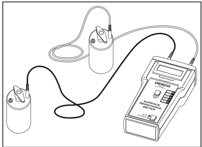
Figure 7. 19780 set up to test resistance point to point.
